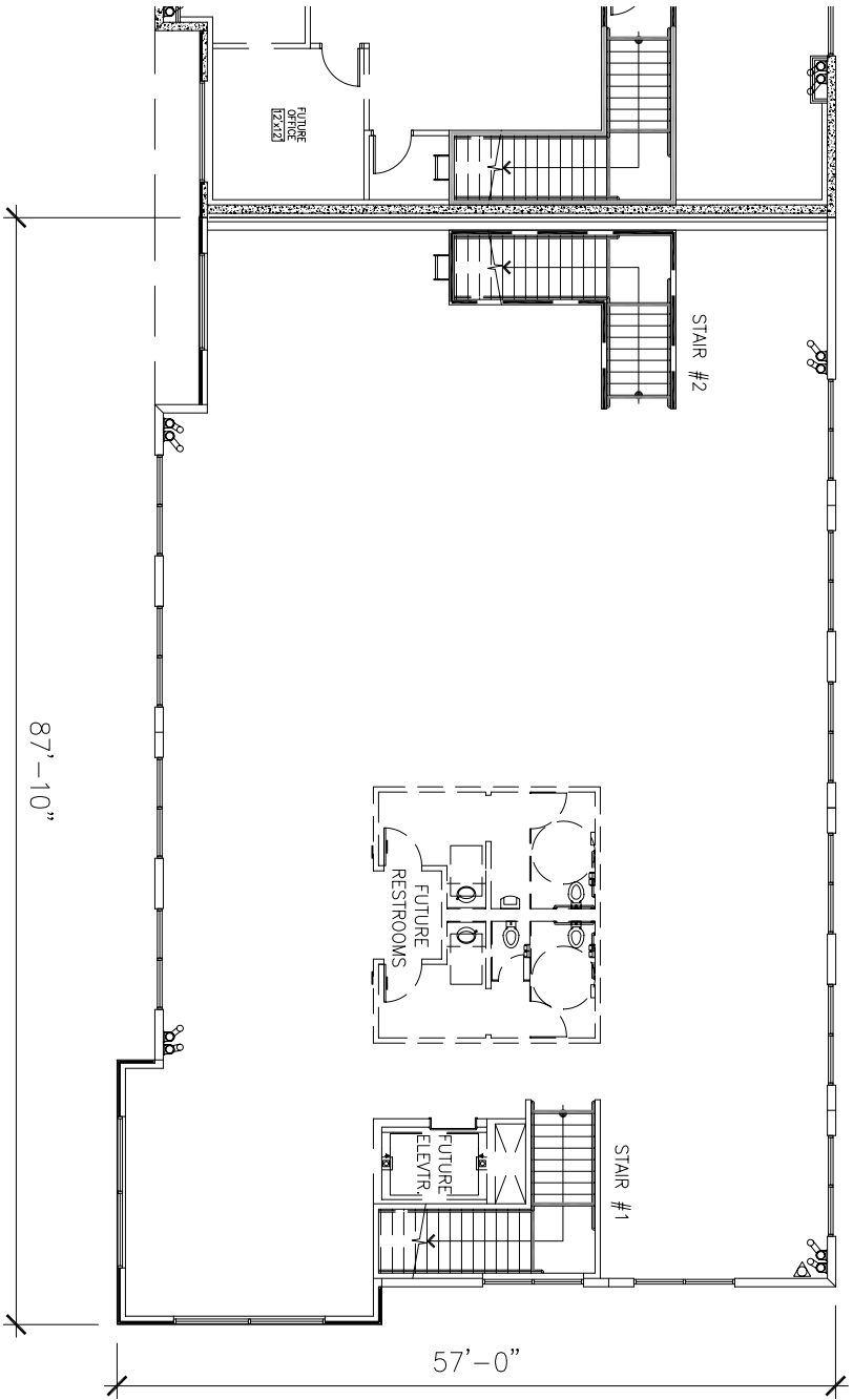
BUILDING 2 - SECOND FLOOR 4,629 S.F.
